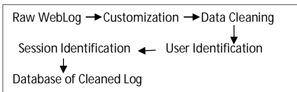
Figure 5: Preprocessing Techniques
