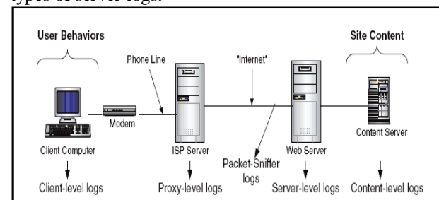
Figure 3: Different types of Logs
